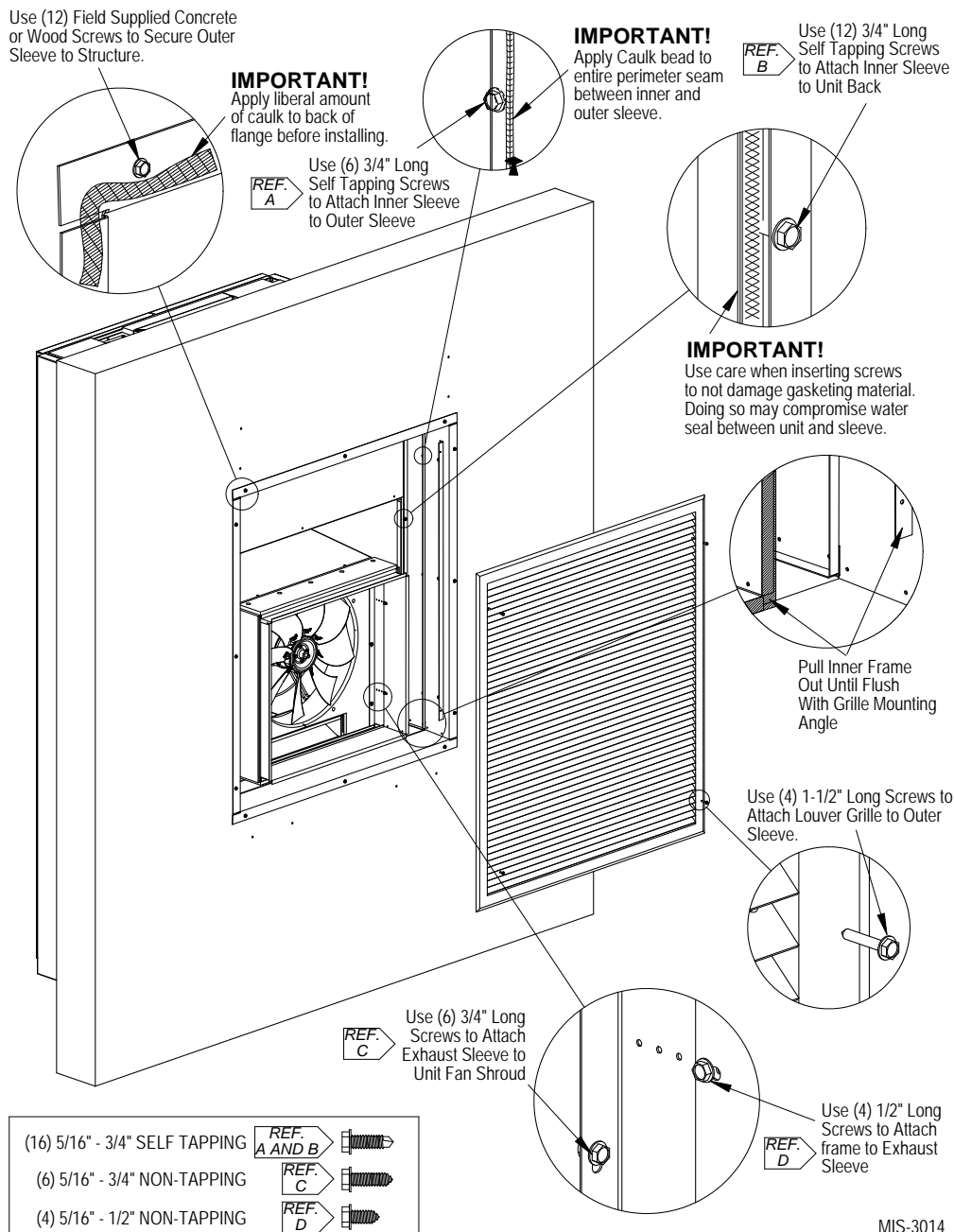
FIGURE 7 ATTACHMENT OF WALL SLEEVE
