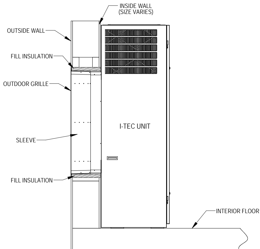
FIGURE 6 TYPICAL INSTALLATION
