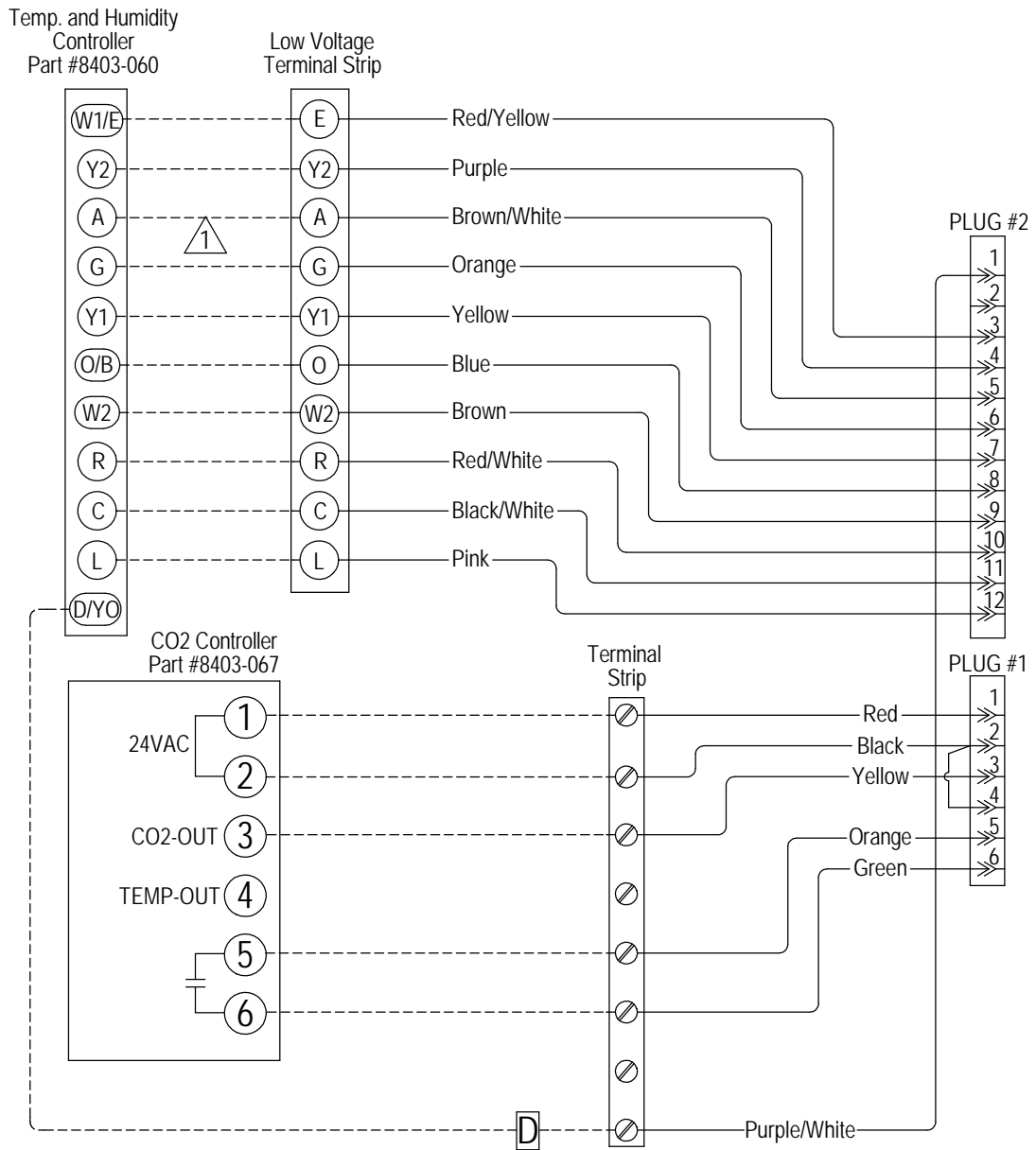
FIGURE 1 8403-060 THERMOSTAT & 8403-067 CO2 CONTROL
