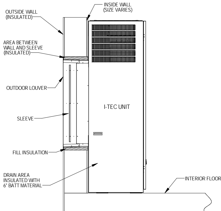
FIGURE 7 Typical Installation
