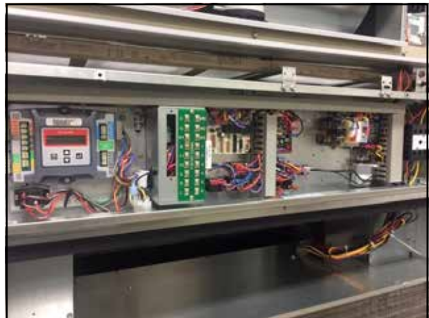
FIGURE 20 Wiring Connections Completed
