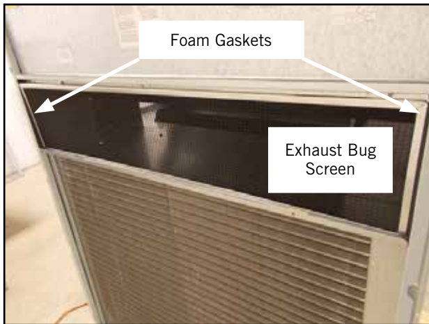
FIGURE 25 Install Bug Screen and Gaskets
