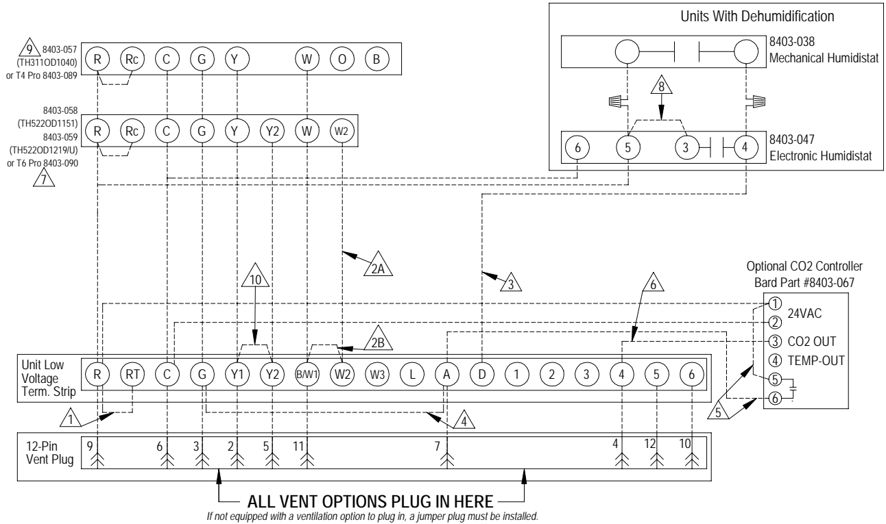
FIGURE 28 Required Control Connections for ECON-**5 with Heat Pumps
