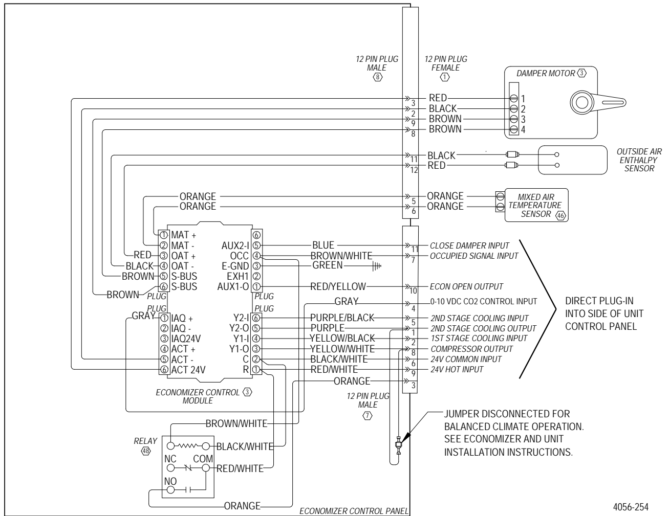
FIGURE 34 Wiring Diagram – Temperature Only Sensor
