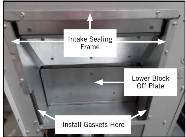
FIGURE 23 Install Intake Sealing Frame and Lower Block Off Plates
