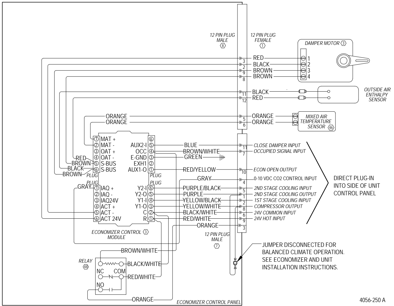
FIGURE 33 Wiring Diagram – Enthalpy Sensor
