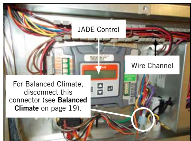
FIGURE 7 Install 910-2063 Control Board Assembly
