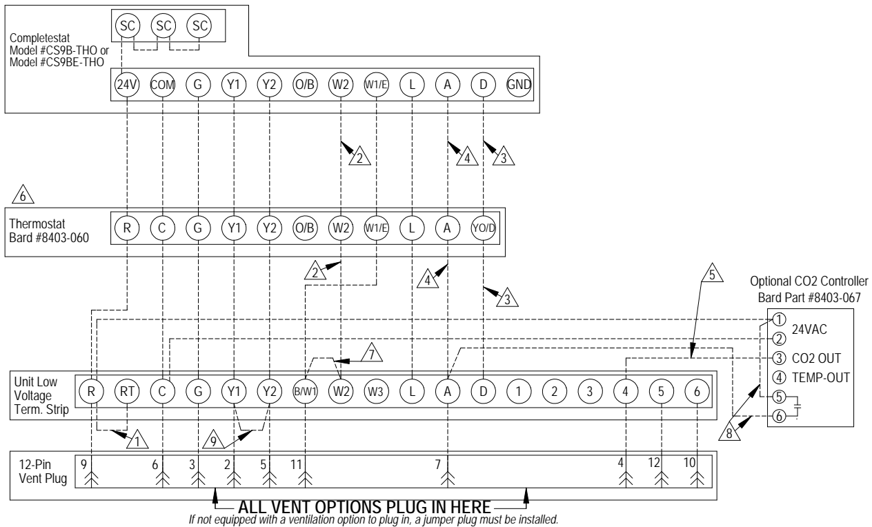
FIGURE 27 Required Control Connections for ECON-**5 with Air Conditioners
