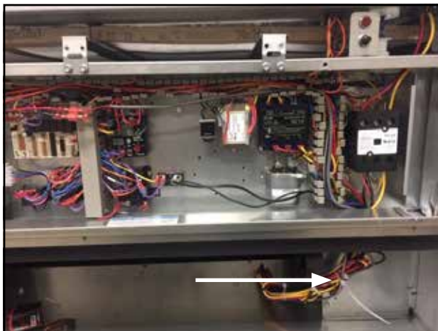
FIGURE 18 Route Cable Through Control Panel Bushing
