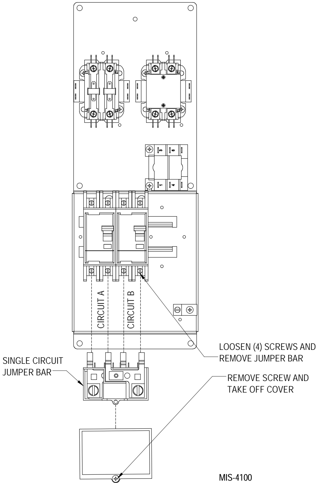
FIGURE 1 Electrical Connections
