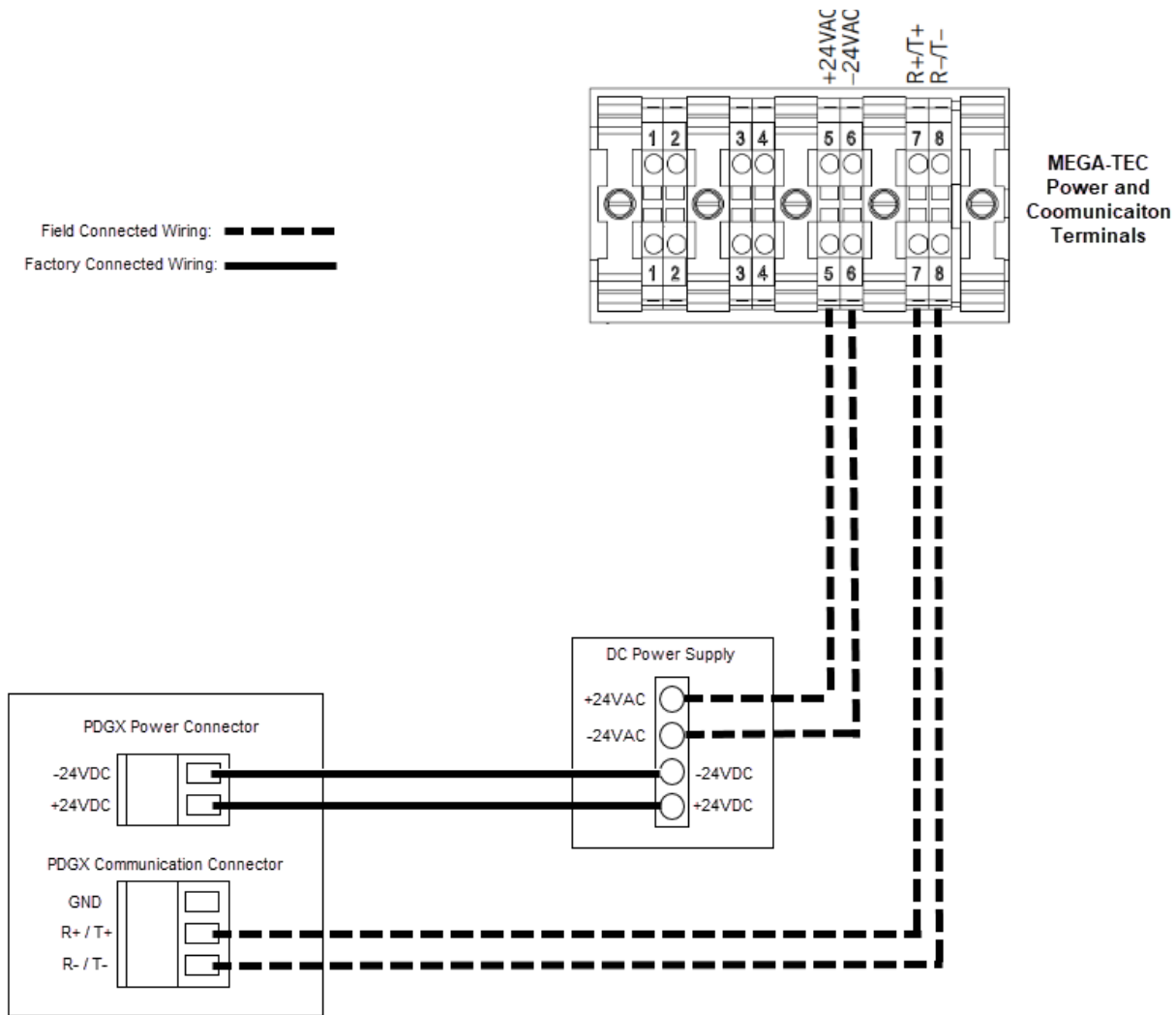
FIGURE 4 Connecting PGDx to MEGA-TEC Unit
