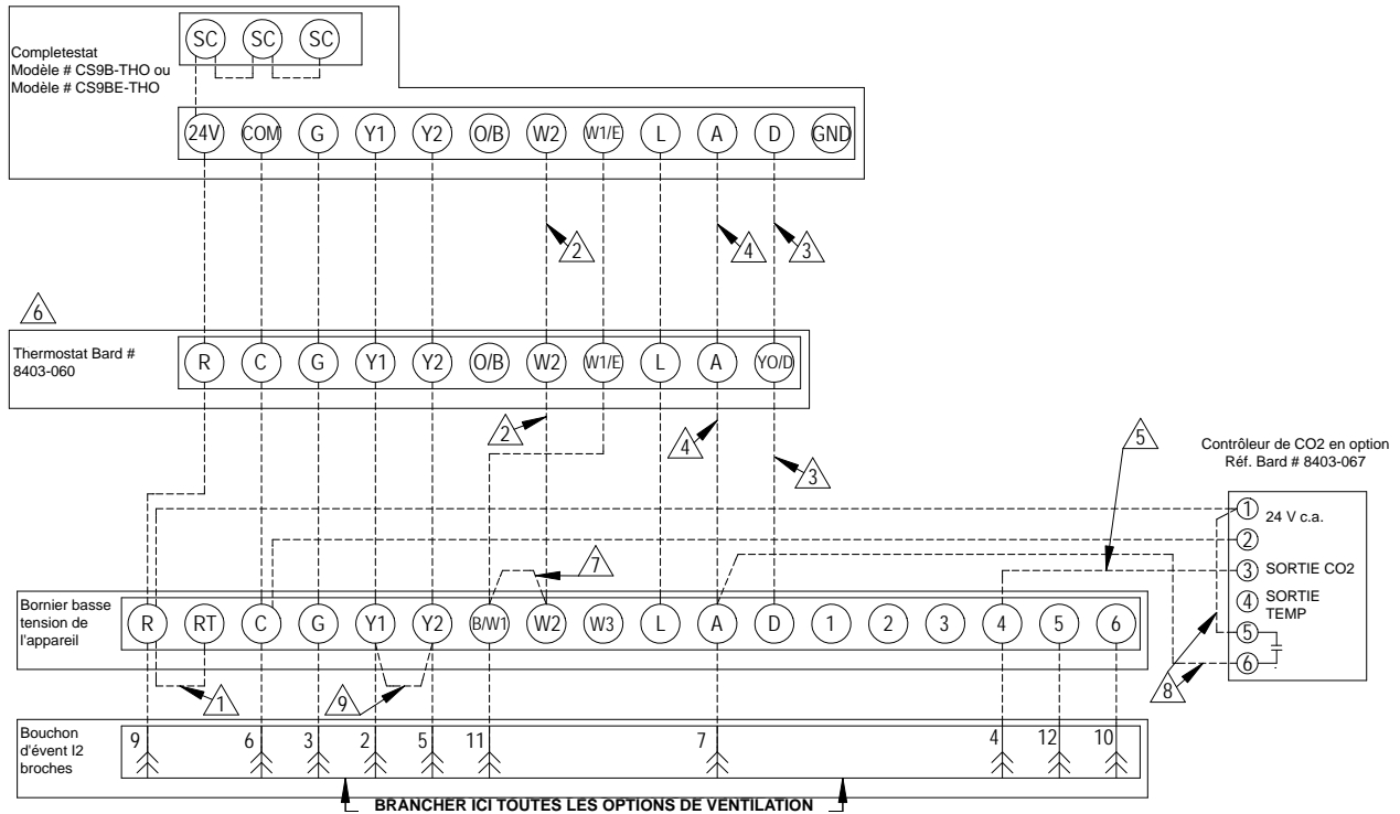
FIGURE 8 Raccords programmables du thermostat
