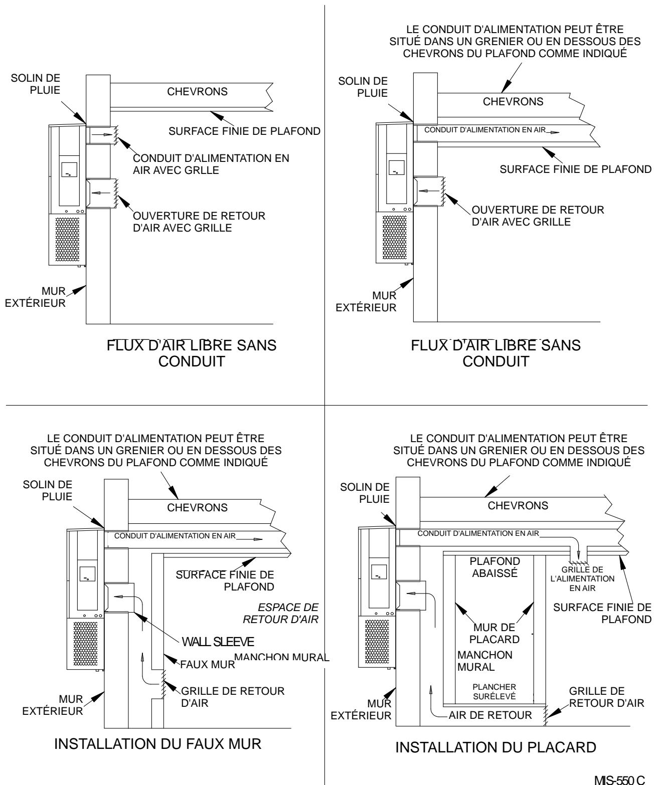
FIGURE 7 Installations murales communes
