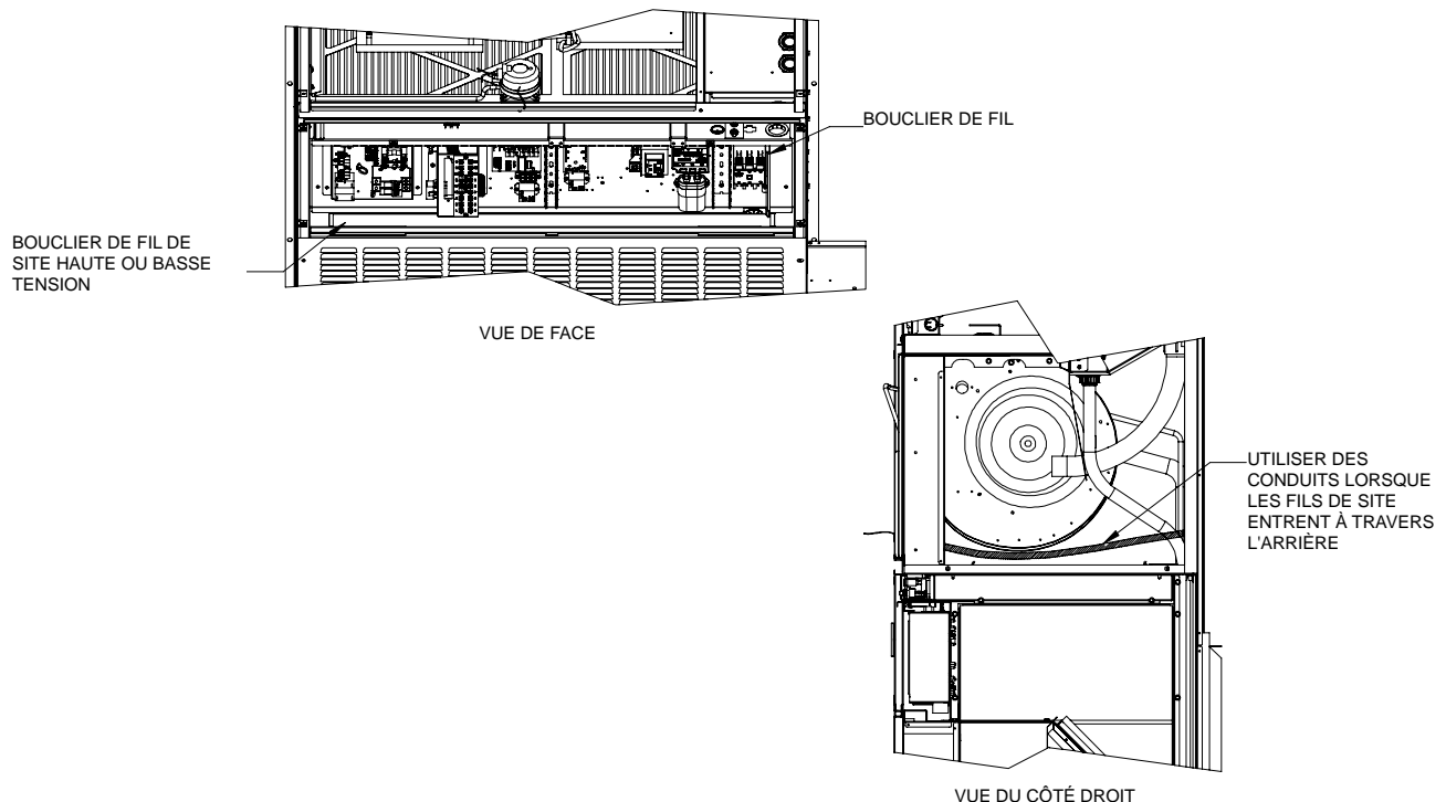
FIGURE 19 Raccords haute tension
