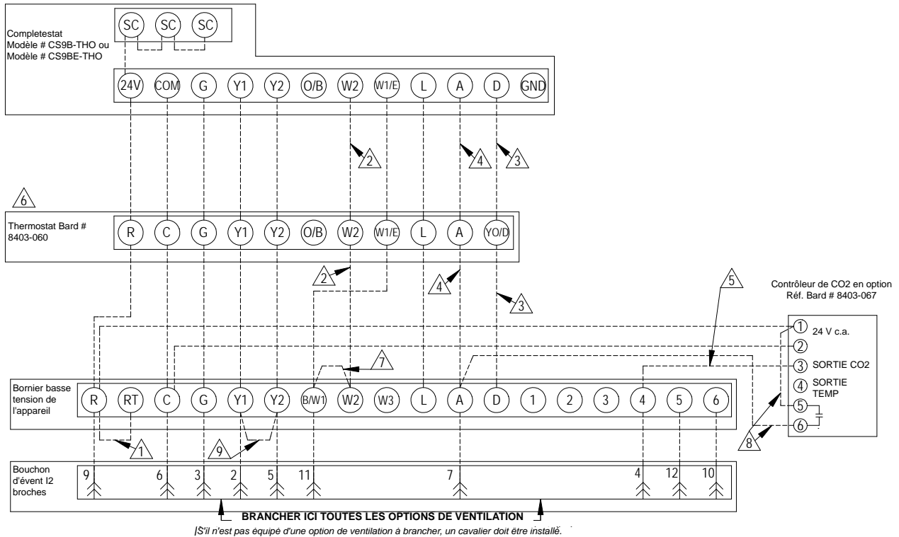
FIGURE 20 Raccords programmables du thermostat
