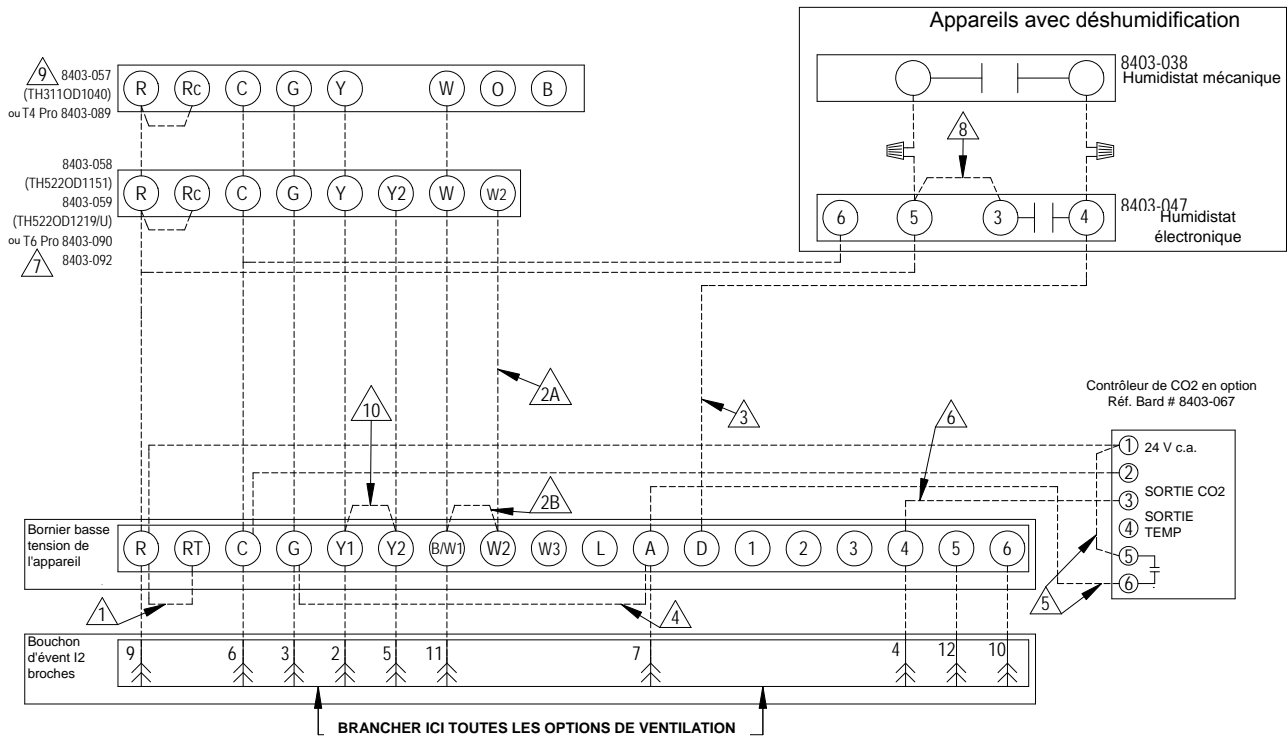
FIGURE 21 Raccords non-programmables du thermostat
