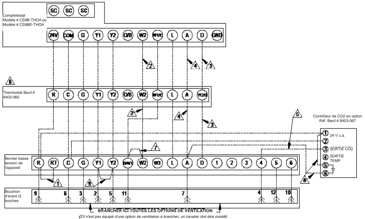
FIGURE 20 Raccordements programmables du thermostat
