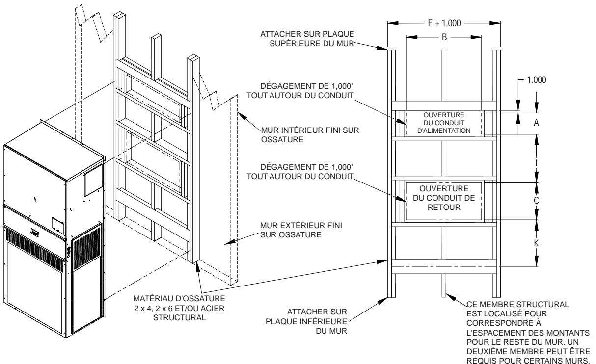
FIGURE 17 Instructions relatives au montage mural
