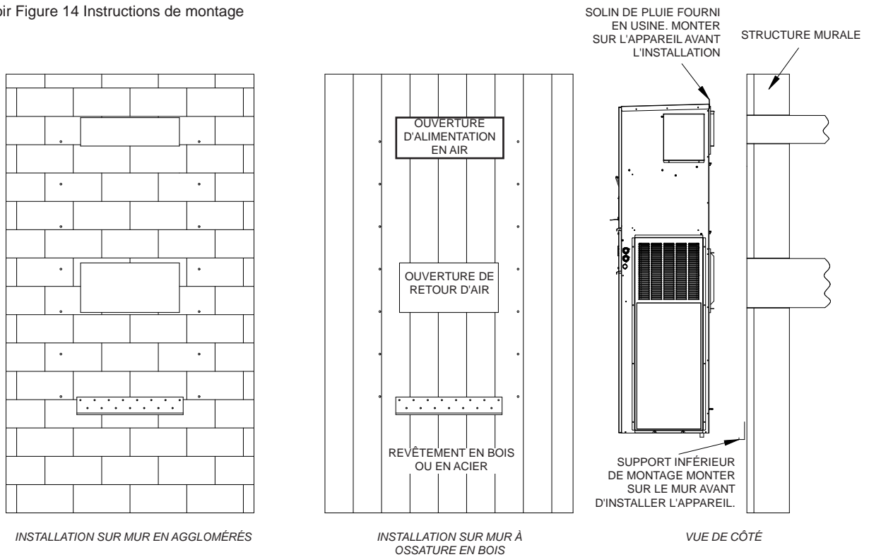
FIGURE 16 Instructions relatives au montage mural
