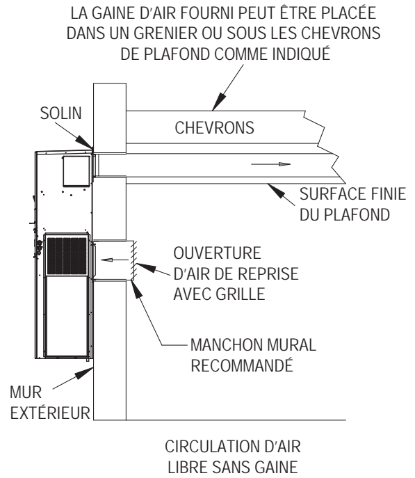
FIGURE 7 Installations murales courantes
