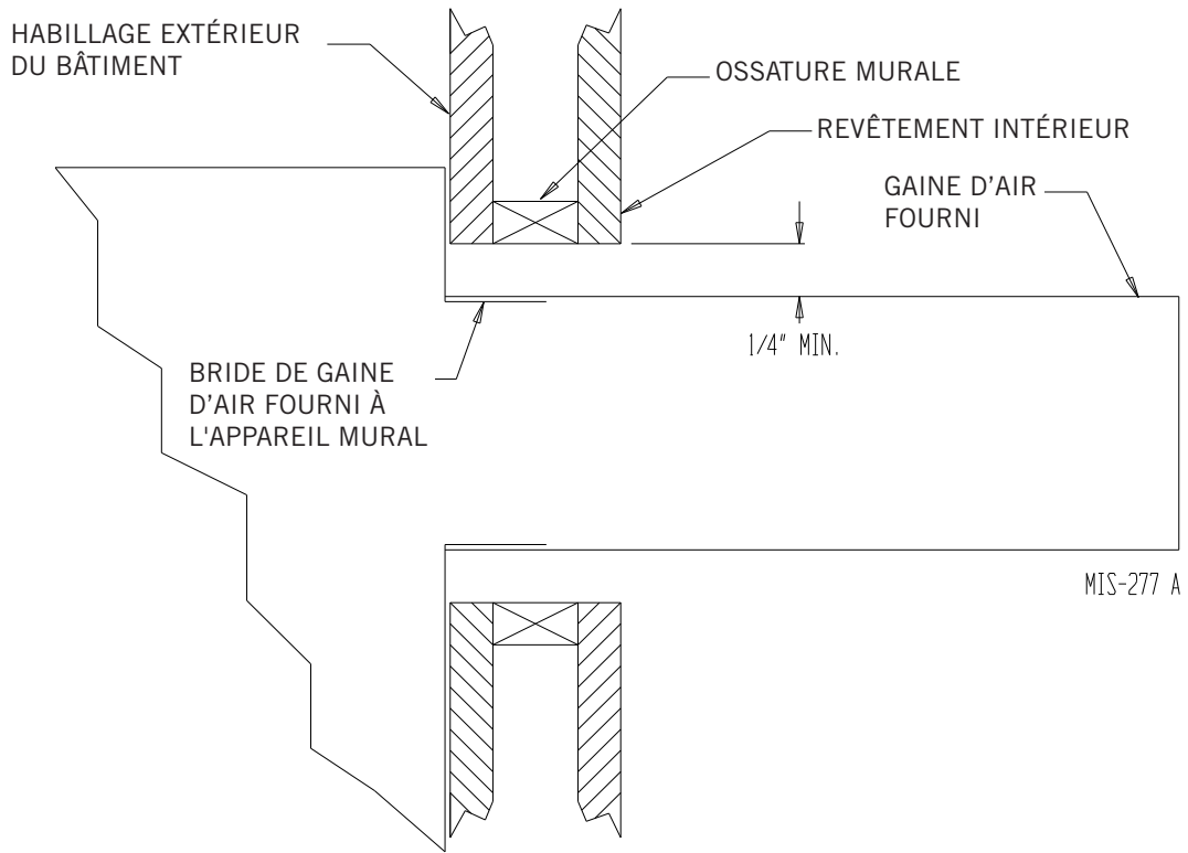
FIGURE 5 Instructions de montage mural
