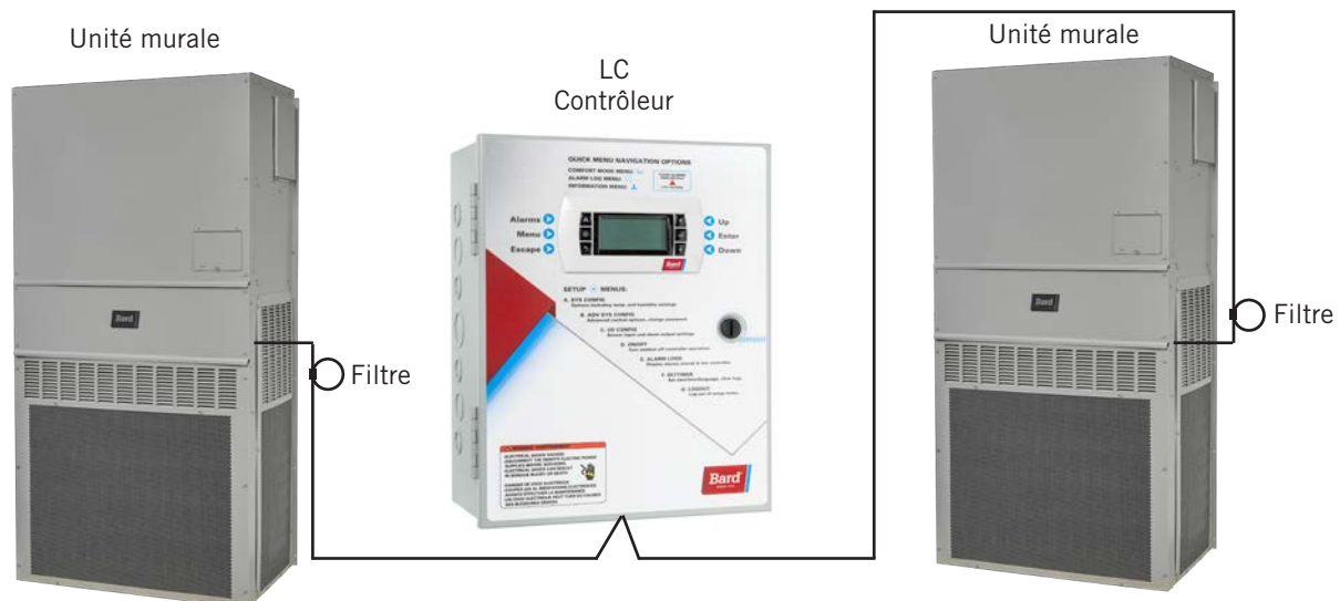
FIGURE 18 Câblage de communication (liaison alternative)
