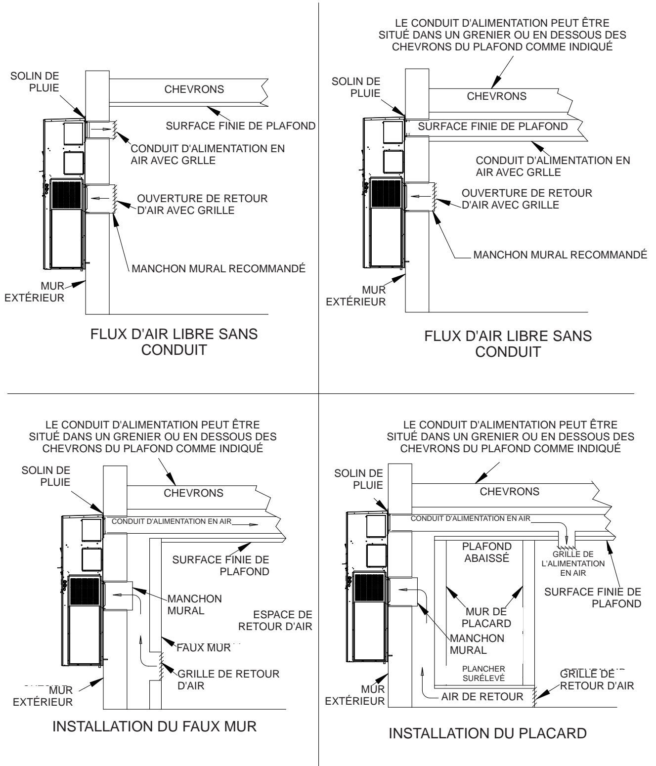
FIGURE 7 Installations murales courantes
