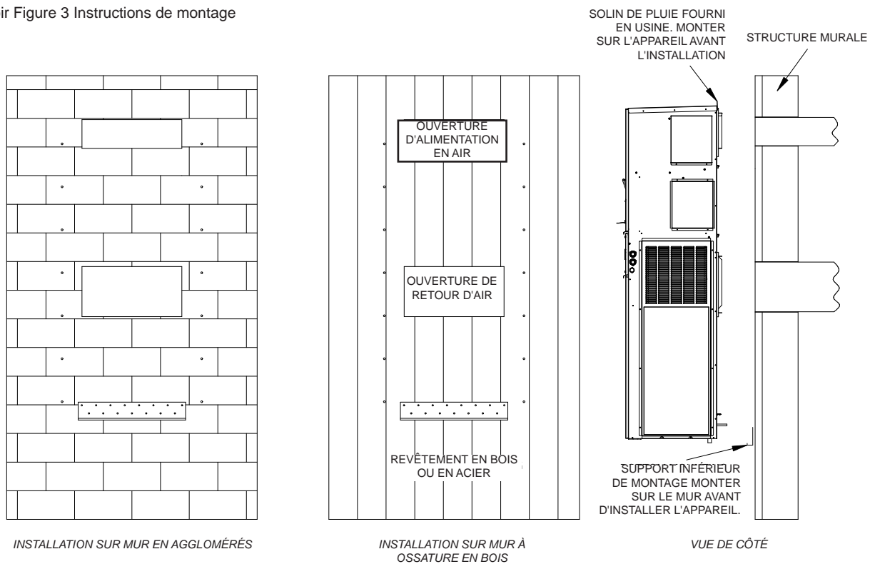
FIGURE 5 Instructions de montage mural
